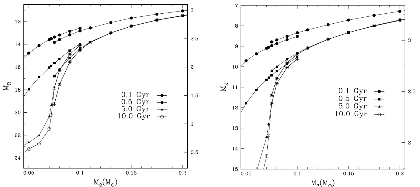
FIG. 7.—Predicted M_R ( left ) and M_K ( right ) as a function of the mass. Isochrones are taken from Baraffe et al. (1998) for masses \geq 0.075 M_\odot and Baraffe et al. (2003) for masses \leq 0.01 M_\odot . The mismatch between isochrones in the range 0.075\text{--}0.01 M_\odot reflect model differences. The axes on the right-hand side are the logarithm of the upper limit to the distance (in pc) toward J00291 given by 5.2 - M_R/5 and 4.7 - M_K/5 (see § 10.3). [See the electronic edition of the Journal for a color version of this figure.]
