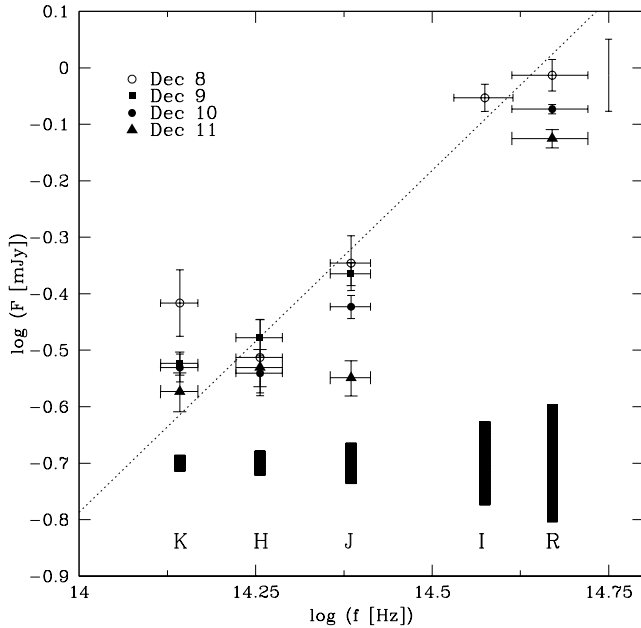
FIG. 4.—Optical/near-infrared spectral energy distribution of J00291 on 2004 December 8, 9, 10, and 11. The fluxes in each band have been dereddened with E(B - V) = 0.8 mag as described in § 7. The error bars of the data are the uncertainties in the photometry, whereas the isolated vertical bar represents the upper limit of the observed flux variation at optical wavelengths. Horizontal error bars are the K_s , H , J , I_C , and R_C filter bandwidths. Overdrawn as bars are the effects in the flux (at the central wavelength of each bandpass) due to the uncertainty ( \pm 0.1 mag) in the reddening. We also show the power-law fit to the December 8 data after excluding the K -band flux (dotted line). The fit yields \alpha = 1.2 \pm 0.2 . [See the electronic edition of the Journal for a color version of this figure.]
