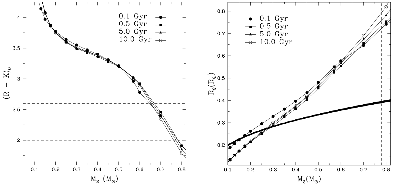
FIG. 6.— Left : Predicted color (R - K) as a function of the mass for low-mass stars with ages 0.1, 0.5, 5, and 10 Gyr. Isochrones are taken from Baraffe et al. (1998). The dashed lines delineate our constraint on the (R - K) quiescent color of J00291. Right : Predicted radius vs. mass diagram for low-mass stars as derived from the isochrones presented in the left panel of the figure. The thick solid line represents the Roche lobe of the donor star when adopting a neutron star mass of 1.4\text{--}2.0 M_\odot . [See the electronic edition of the Journal for a color version of this figure.]
