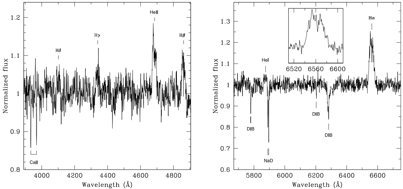
FIG. 3.—Normalized and averaged optical spectrum of J00291. Major disk and interstellar features are identified. DIB denotes the diffuse interstellar bands. The inner panel shows a zoom of the averaged H \alpha emission line profile.
