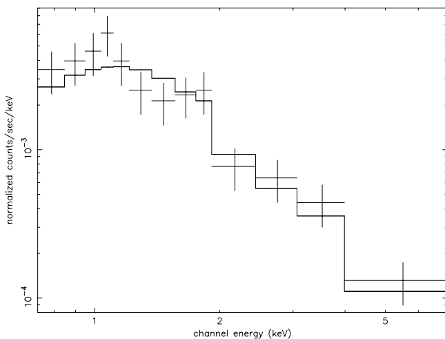
FIG. 5.—X-ray spectrum of J00291 obtained during quiescence. The solid line through the spectrum is the best-fit absorbed power-law model with N_{\text{H}} = 4.6 \times 10^{21} \text{cm}^{-2} .
