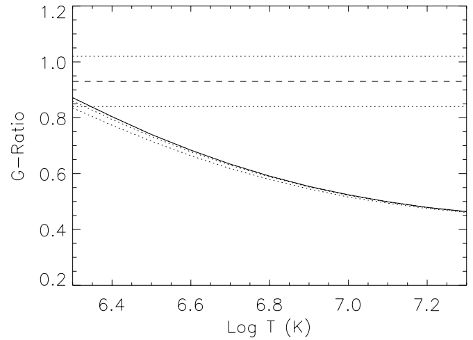
FIG. 11.—Determination of the plasma temperature from the G -ratio for the fluxes adjusted for line blending (dashed line). Errors on the measured ratio are represented by dotted lines. APEC models are given for 10^{10}, 10^{11}, 10^{12}, and 10^{13} \text{ cm}^{-3} , with the solid curve denoting the 10^{10} \text{ cm}^{-3} (i.e., low-density) model.
