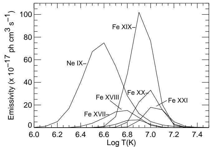
FIG. 13.—Total emissivities as functions of temperature for each ion emitting strong lines in the wavelength range between 13.35 and 13.85 Å. Calculations are APEC models for solar abundances and low density. Table 5 gives the wavelengths for the lines identified in this work.
