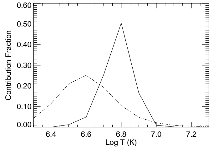
FIG. 12.—Fraction of Ne IX resonance line emission arising from each temperature in the plasma (solid curve), derived by multiplying the emission measure distribution of Fig. 7 with the fractional emissivity curve from APEC (dot-dashed line). The intercombination and forbidden lines have virtually the same dependences and are not shown.
