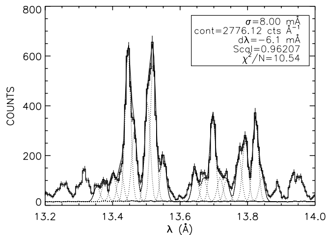
FIG. 4.—HEG summed spectrum of Capella using plus and minus first order. In order to construct an empirical model, 18 emission lines are used with Gaussian line widths \sigma = 0.005 \text{ \AA} (equivalent to FWHM = 0.012 \text{ \AA} ). The continuum level (including weak lines and background, for combined plus and minus first orders) is chosen constant with 700 counts \text{\AA}^{-1} . The bin size is 2.5 \text{ m\AA} , and the exposure time is 154.7 ks.
