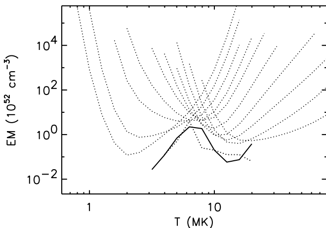
FIG. 7.—Best-fit emission measure distribution derived from iron lines in ionization stages Fe xv to Fe xxiv (solid line). The result from Brickhouse et al. (2000) is also shown (lower dotted line). Individual line emission measure curves (upper dotted lines) are shown for the lines in Table 6.
