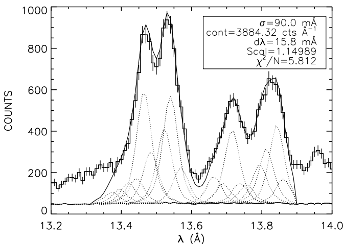
FIG. 5.—Best-fit model obtained from the HEG spectrum, scaled and overlaid on the measured spectra from MEG (top) and LETGS (bottom). The scaling parameters d\lambda , Scal , \sigma , and cont (described in the text) are listed in the top right inset. The goodness of fit \chi^2/N is also given. For MEG the bin size is 5.0 \text{ m\AA} , and the exposure time is 154.7 ks. For LETGS the bin size is 10.0 \text{ m\AA} , and the exposure time is 218.5 ks.
