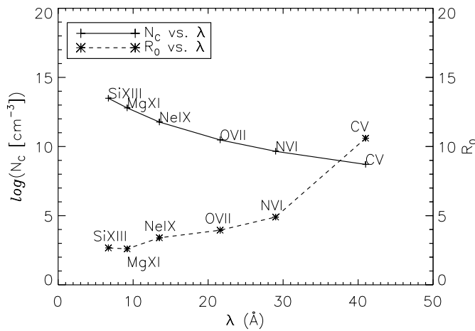
FIG. 1.—Low-density limits R_0 and critical densities N_c for the different He-like ions showing systematic, anticorrelated trends with wavelength, due ultimately to the nuclear charge (from Pradhan & Shull 1981; Blumenthal et al. 1972). Large R_0 (C v) implies that the i flux may be difficult to measure. Large N_c may be outside the interesting coronal range (Si XIII). Ne IX appears to have ideal values for coronal physics.
