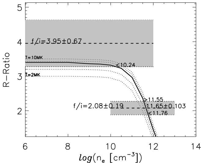
FIG. 10.—Determination of the plasma density from the R -ratio using f and i from the direct measurement ( f/i = 2.1 \pm 0.2 ) and from the model accounting for line blends ( f/i = 3.9 \pm 0.7 ). Shaded areas represent 1 \sigma errors on the measured ratios. The upper limit for the density is \log n_e < 10.2 . APEC models for the density-sensitive curves are shown for T = 2.0, 4.0, 6.3, 8.0, and 10 MK, with the curve denoting the 6.3 MK model corresponding to the peak of the emission measure distribution. The R -ratio increases with temperature.
