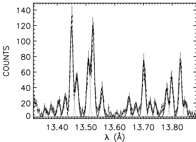
FIG. 4.—HEG summed spectrum of Capella using plus and minus first order. In order to construct an empirical model, 18 emission lines are used with Gaussian line widths \sigma = 0.005 \text{ \AA} (equivalent to FWHM = 0.012 \text{ \AA} ). The continuum level (including weak lines and background, for combined plus and minus first orders) is chosen constant with 700 counts \text{\AA}^{-1} . The bin size is 2.5 \text{ m\AA} , and the exposure time is 154.7 ks.
