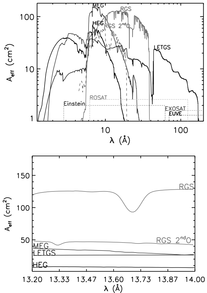
FIG. 2.—Effective areas for the Chandra and XMM-Newton gratings, with ranges of other observatories shown as dotted lines. At 13.6 Å, the RGS has the largest area, while HEG is the least sensitive. The bottom panel shows detail in the Ne IX region.
