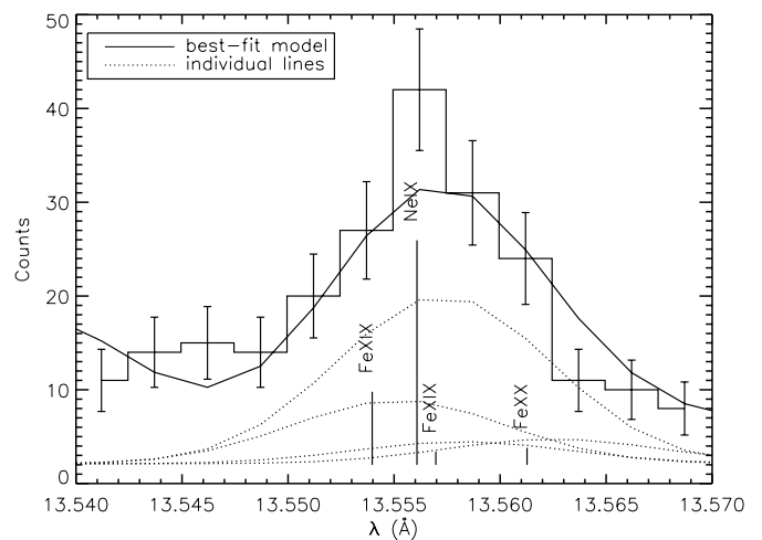
FIG. 9.—Same as Fig. 8, but in more detail, showing the Ne IX intercombination line with contamination.
