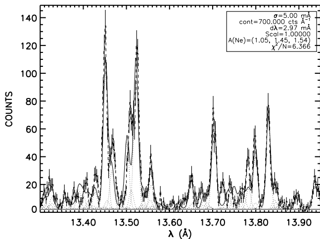
FIG. 8.—Measured spectrum of Capella obtained from HEG ( histogram with error bars ), APEC individual predicted emission lines ( dotted lines ), and their sum ( thick solid line ). Predicted line fluxes were estimated using the emission measure distribution described in § 4.2. Bin size is 2.5 mÅ, and exposure time is 154.7 ks.
