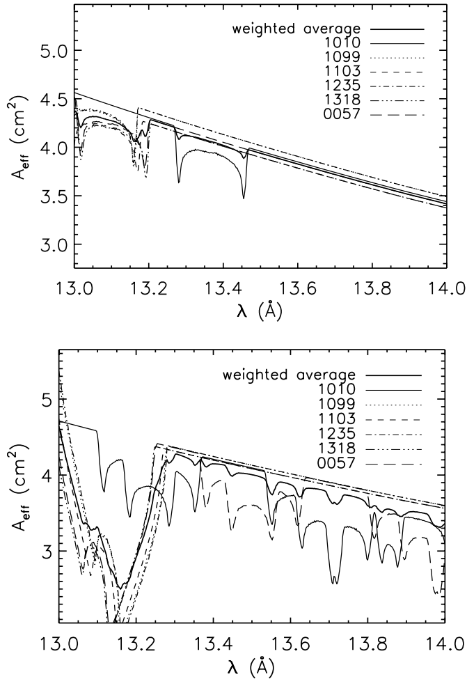
FIG. 3.—Effective areas for the different observations (labeled with observation identification) with the HEG plus first order ( top ) and minus first order ( bottom ). The average is indicated by a thick line and is obtained by weighting with the exposure times. The large dip on the short-wavelength end of the minus first order is the chip gap, while smaller dips are caused by the removal of bad pixels. The widths and shapes of these dips are determined by the aspect dither and the chip geometry.
