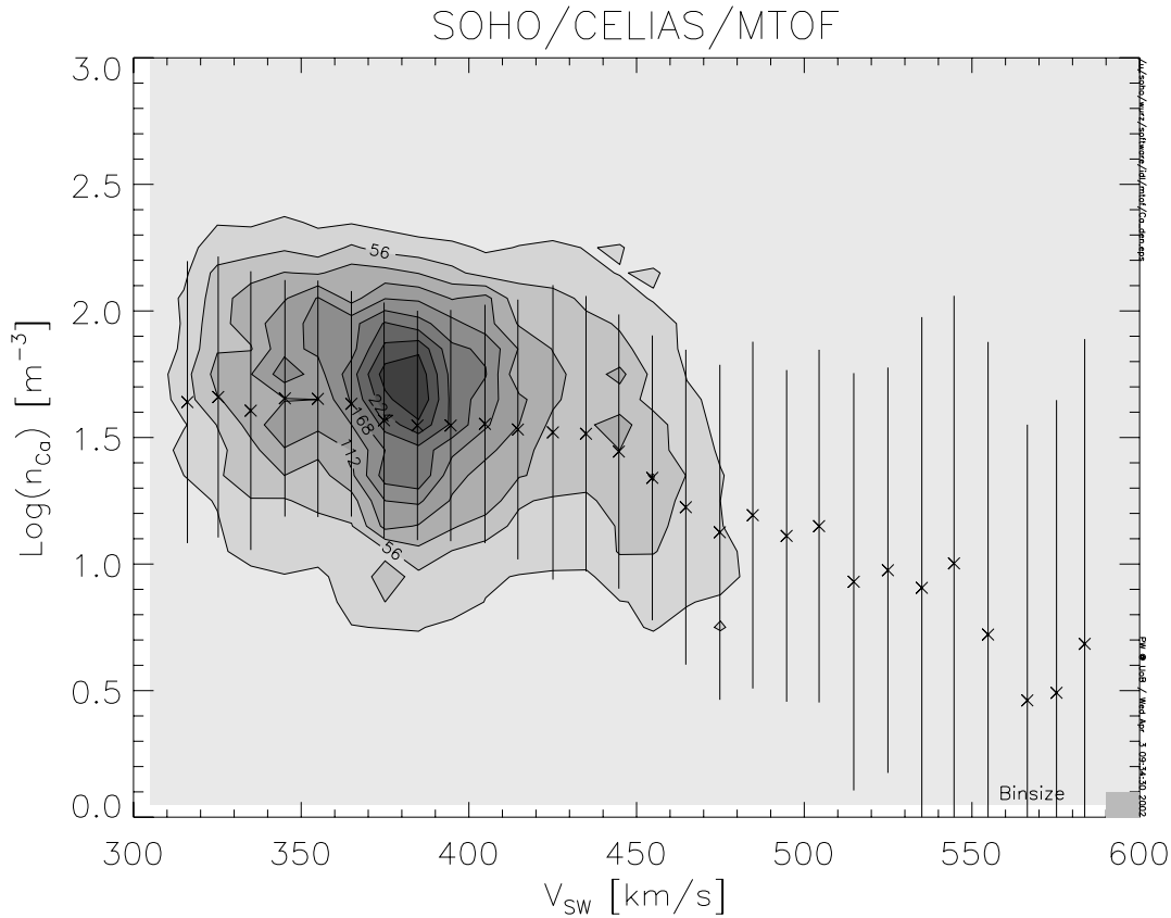
FIG. 3.—Logarithm of calcium densities measured with CELIAS/MTOF at 1 AU vs. the solar wind velocity. Ten linearly spaced contours: Number of measurements for a particular bin. Data have been selected from DOY 30 through DOY 366 of 1996. During that time period, there was mostly slow solar wind, which explains the clustering of measurements between 300 and 400 km s -1 . Crosses: Mean for a particular velocity bin. Error bars: Standard deviation of log( N_{Ca} ) for a single measurement. [See the electronic edition of the Journal for a color version of this figure.]
