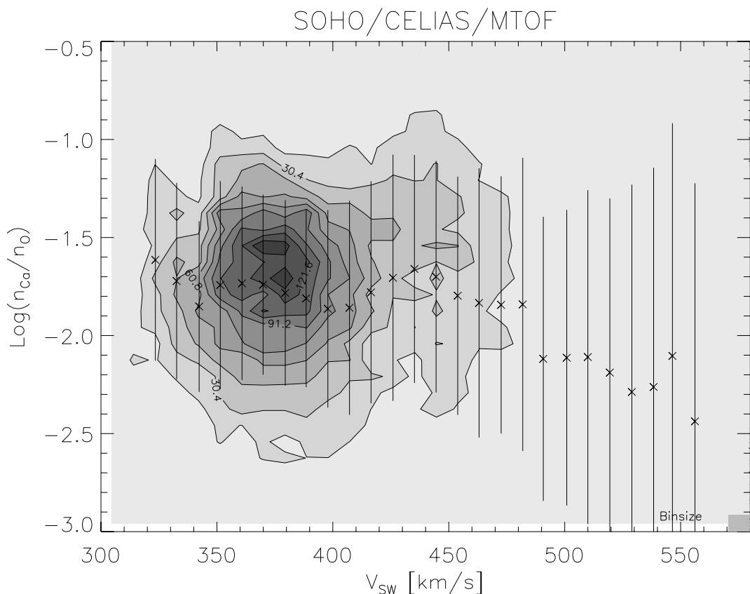
FIG. 4.—Logarithm of calcium to oxygen abundance ratio measured with CELIAS/MTOF at 1 AU vs. the solar wind velocity. Ten linearly spaced contours: Number of measurements for a particular bin. Data have been selected from DOY 30 through DOY 366 of 1996. During that time period, there was mostly slow solar wind, which explains the clustering of measurements between 300 and 400 km s -1 . Crosses: Mean for a particular velocity bin. Error bars: Standard deviation of log( N_{Ca}/N_O ) for a single measurement. [See the electronic edition of the Journal for a color version of this figure.]
