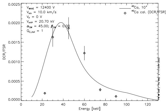
FIG. 1.—Calibration data from the MTOF flight-spares sensor for Ca (symbols) and the result of the instrument function (line). DCR/FSR stands for the double-coincidence rate vs. the start rate of the TOF section of the MTOF sensor.
