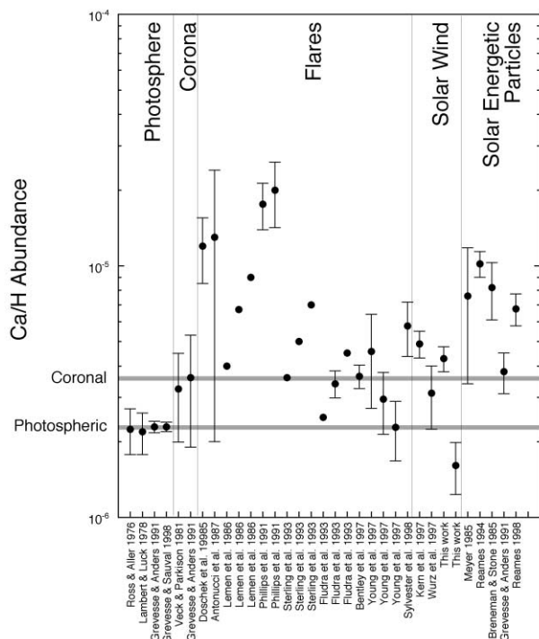
FIG. 5.—Summary of published Ca abundance measurements. Lower gray line: Photospheric Ca abundance. Upper gray line: Coronal Ca abundance. See text and Table 1 for details.
