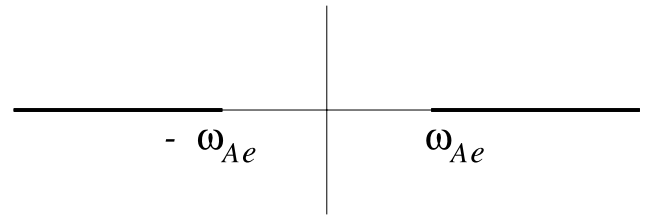
FIG. 2.—Complex \omega -plane with two cuts shown by the bold lines. The function \zeta_e(\omega) is single-valued in this plane. Similar cuts in the complex \omega -plane, although from -\omega_{Ae} and \omega_{Ae} , are used to make the functions \zeta_i(\omega) single-valued.
