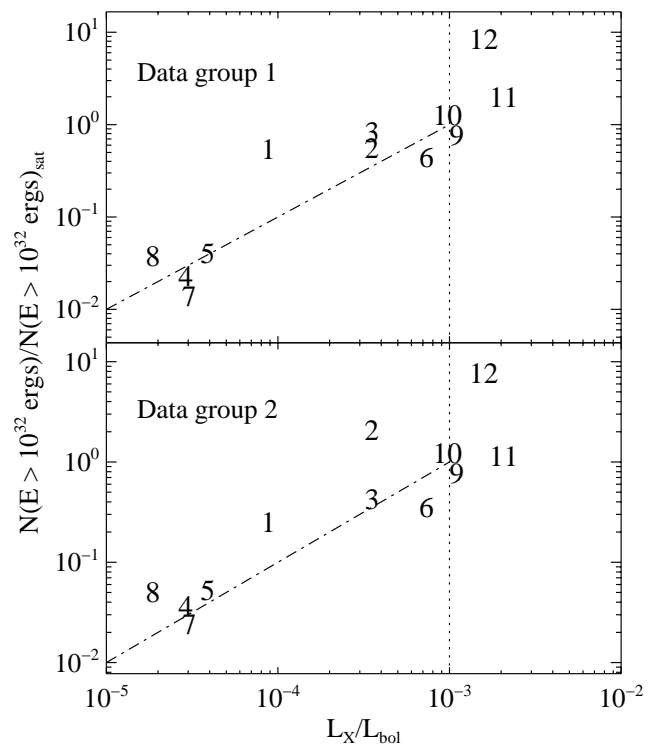
FIG. 6.—Normalized occurrence rate of flares with energies larger than 10^{32} ergs vs. ratio L_X/L_{\text{bol}} of the coronal luminosity and the bolometric luminosity. Data groups 1 and 2 are identical to Fig. 4. The numbers are as in Fig. 5. The dash-dotted lines are lines with slope 1. The dotted lines represent the saturation level ( L_X = 10^{-3}L_{\text{bol}} ). Note that, for clarity, the N(>E_c) of points 4 and 9 have been multiplied and divided by a factor of 1.5, respectively.
