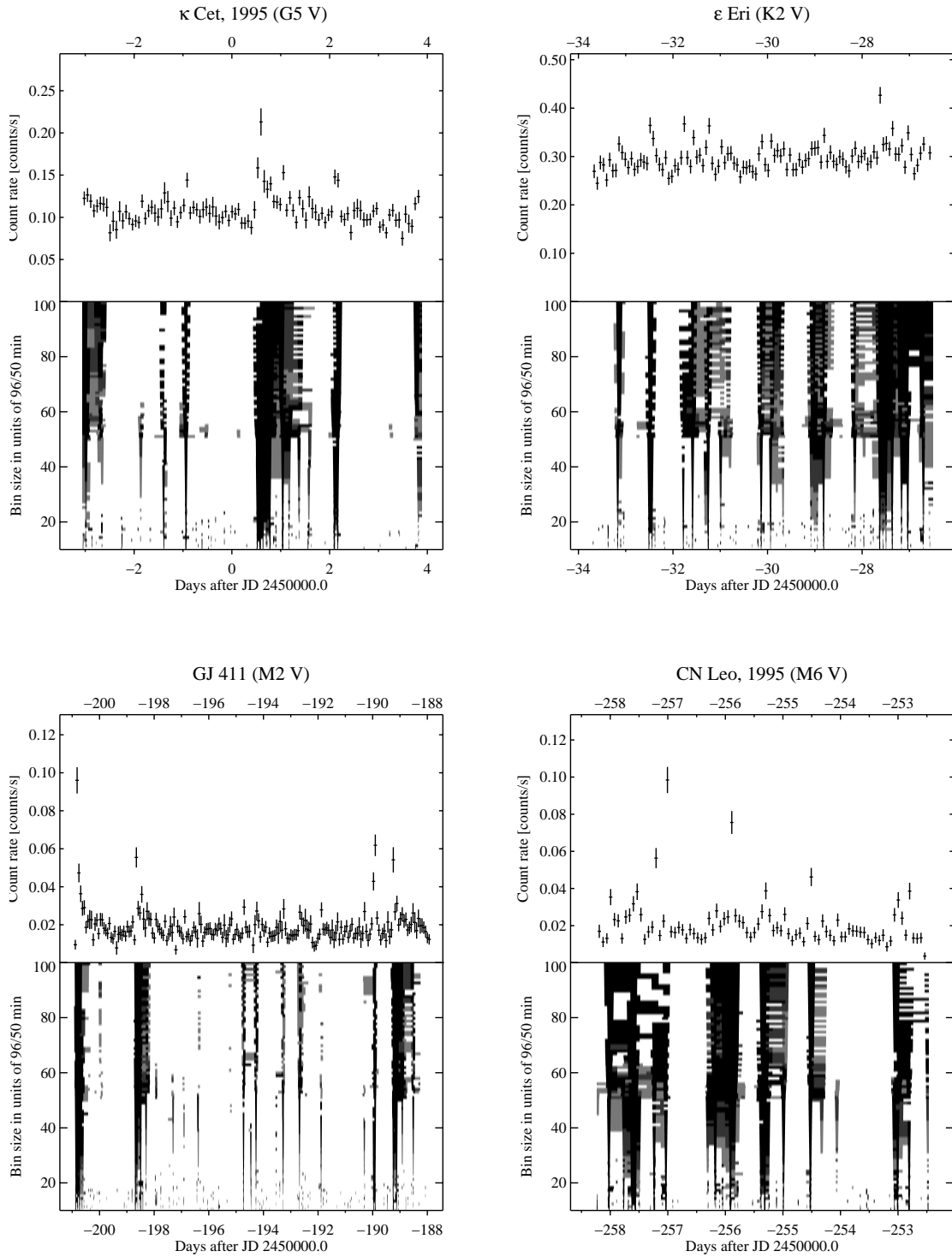
FIG. 1.—Examples of light curves and significance plots
