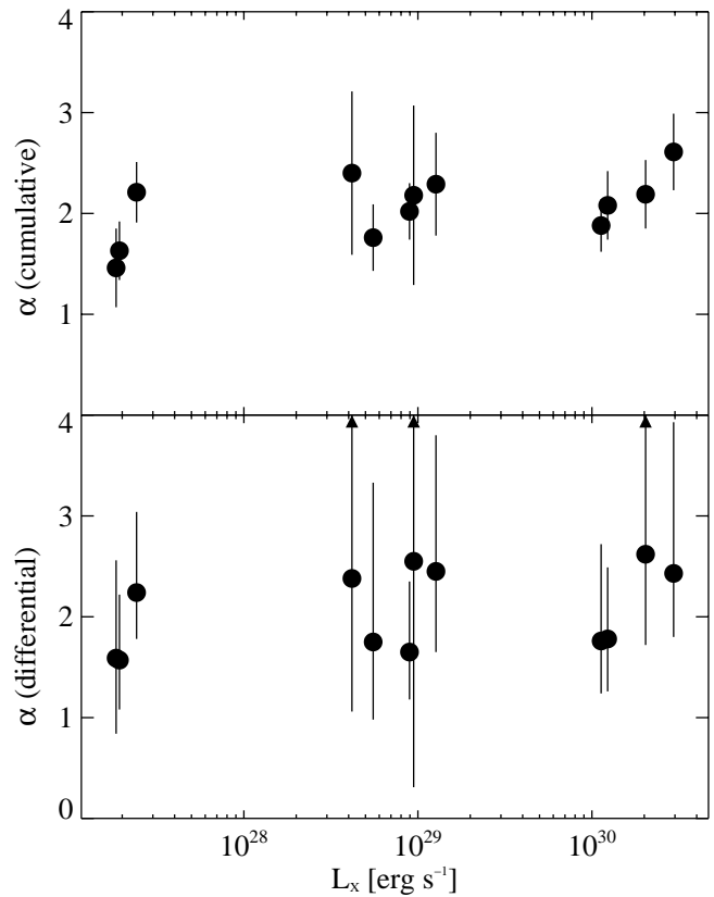
FIG. 3.—Power-law index \alpha vs. coronal L_X
