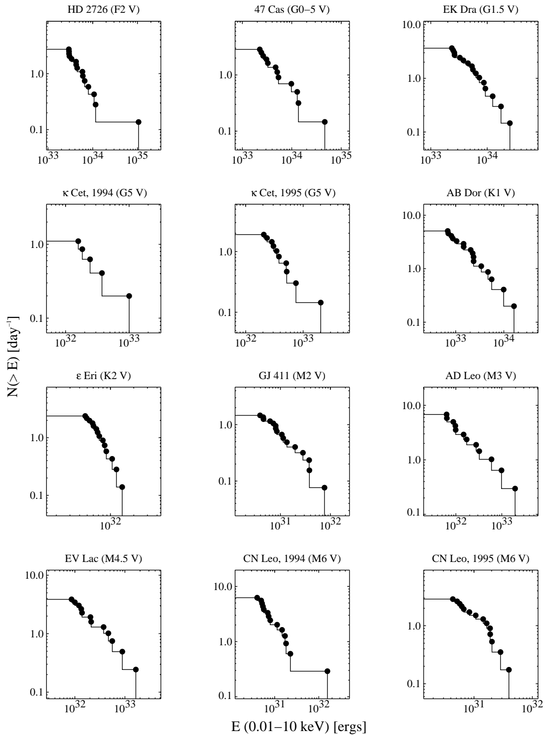
FIG. 2.—Cumulative flare occurrence rate distributions for all 12 data sets
