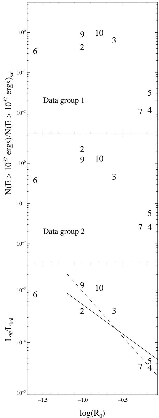
FIG. 8.—(Upper and middle panels) Normalized flare rate vs. Rossby number. Data groups and identifications are as in Fig. 5. (Lower panel) Ratio L_X/L_{\text{bol}} vs. the Rossby number for our sample. The solid line corresponds to the fit by Randich et al. (1996), while the dashed line refers to our best fit (see text).
