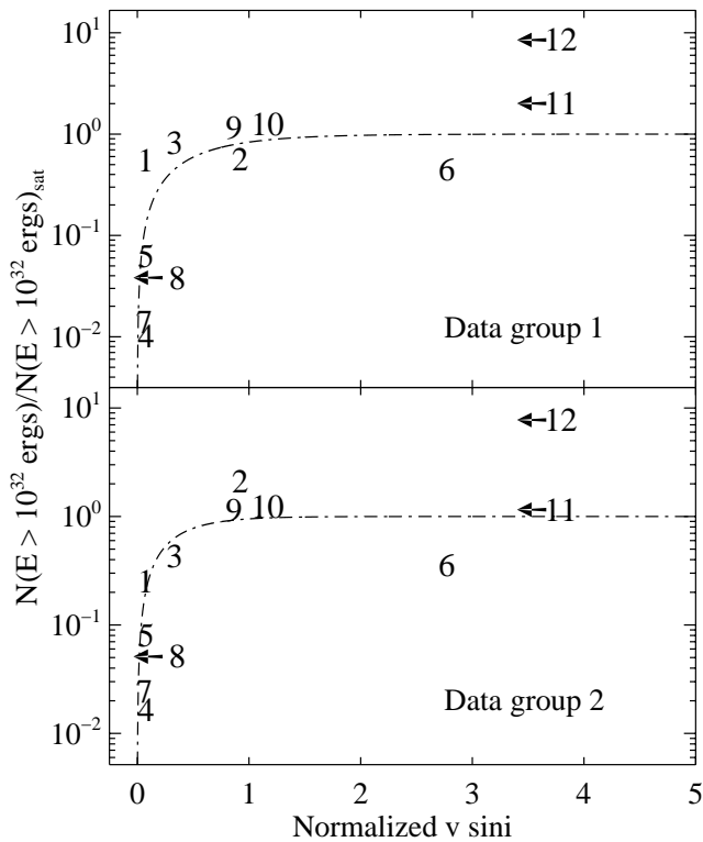
FIG. 7.—Normalized occurrence rate of flares with energies larger than 10^{32} ergs vs. normalized projected rotational velocity v \sin i / (v \sin i)_{\text{sat}} = x (spectral-type dependent). Data groups 1 and 2 are identical to Fig. 4. “Saturation” fits of the form 1 - \exp(-x/\zeta) are plotted as dot-dashed lines. Arrows indicate upper limits. Note that, for clarity, the N(> E_c) of points 4 and 5 have been divided and multiplied by a factor of 1.5, respectively.
