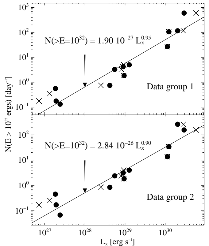
FIG. 4.—Occurrence rate of flares with energies larger than 10^{32} ergs vs. coronal luminosity L_X . Data group 1 corresponds to the rates derived from the fits to cumulative distributions, while data group 2 corresponds to the rates derived from the fits to differential distributions. The \chi^2 linear best fits in the log-log plane are shown as straight lines together with the analytical formulation. Crosses represent L_X values for these sources taken from the literature (see text).
