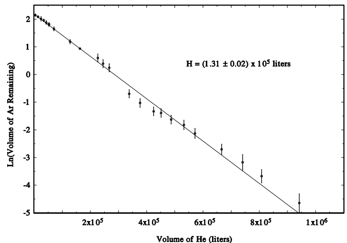
FIG. 6.—Removal of air argon. Amount of air argon remaining in the \text{C}_2\text{Cl}_4 tank as function of the volume of helium that flowed through the system during the initial purge. The response of the system does not deviate from an exponential for over 3 orders of magnitude.
