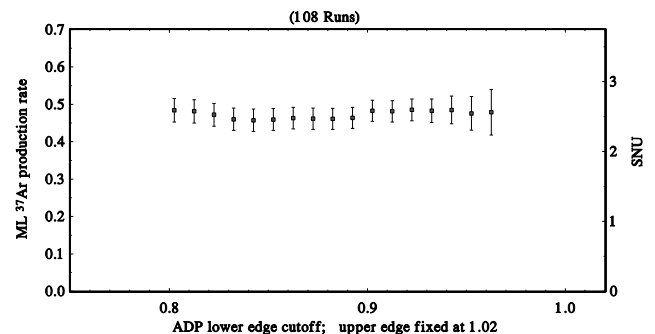
FIG. 12.—Results: variable ADP selection. Average SNU rate for the Homestake detector, as a function of the low edge of the normalized ADP acceptance region; the high edge is fixed at 1.02 (see Fig. 10).
