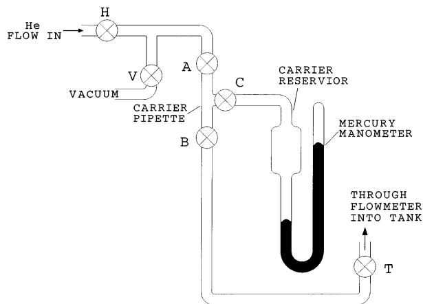
FIG. 3.—Carrier argon measurement and insertion apparatus. This schematic shows the apparatus used to measure and insert a volume of isotopically enriched argon carrier into the C 2 Cl 4 tank, which is used to determine the extraction efficiency (as described in § 4.3). There are two such devices attached to the system, one for 36 Ar and a second for 38 Ar.
