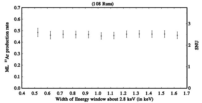
FIG. 11.—Results: variable energy selection. Average SNU rate for the Homestake detector, as a function of the width (about 2.8 keV) of the energy acceptance region for ^{37}\text{Ar} events in the proportional counter. The smallest acceptance region runs from 2.55 to 3.05 keV (0.5 keV width); the largest is from 2.0 to 3.6 keV (1.6 keV width) (see Fig. 9).
