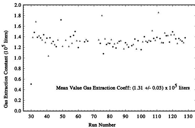
FIG. 4.—Gas extraction coefficients. Value of the extraction constant H , determined for each run by the method described in Appendix A.
