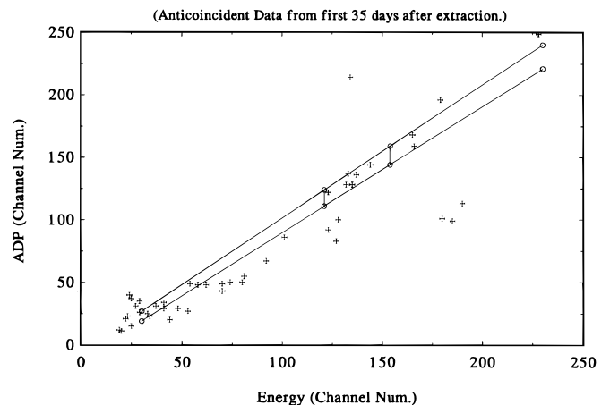
FIG. 8.—ADP vs. energy. (Energy, ADP) of each of the nonvetoed pulses of run 130 that occurred during the first 35 days of counting, together with the energy and ADP bounds of the acceptance region determined by the ^{53}\text{Fe} calibration. The diagonal lines mark the fast region; the vertical lines indicate the one FWHM region about the 2.82 keV energy of the ^{37}\text{Ar} decay.
