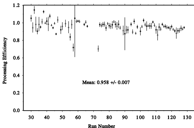
FIG. 5.—Processing efficiency for each extraction, as determined by the method described in Appendix A.
