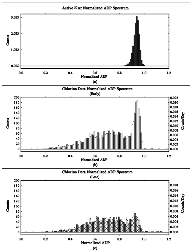
FIG. 10.—(a) ADP spectrum from a counter filled with active ^{37}\text{Ar} . (b) Cumulative ADP spectrum from 93 solar neutrino observations (early counting data: 0–105 days following the end of an extraction). (c) Cumulative ADP spectrum from 93 solar neutrino observations (late counting data: 175–350 days following the end of an extraction). Plots (b) and (c) are of events with energy between 2.0 and 3.6 keV.
