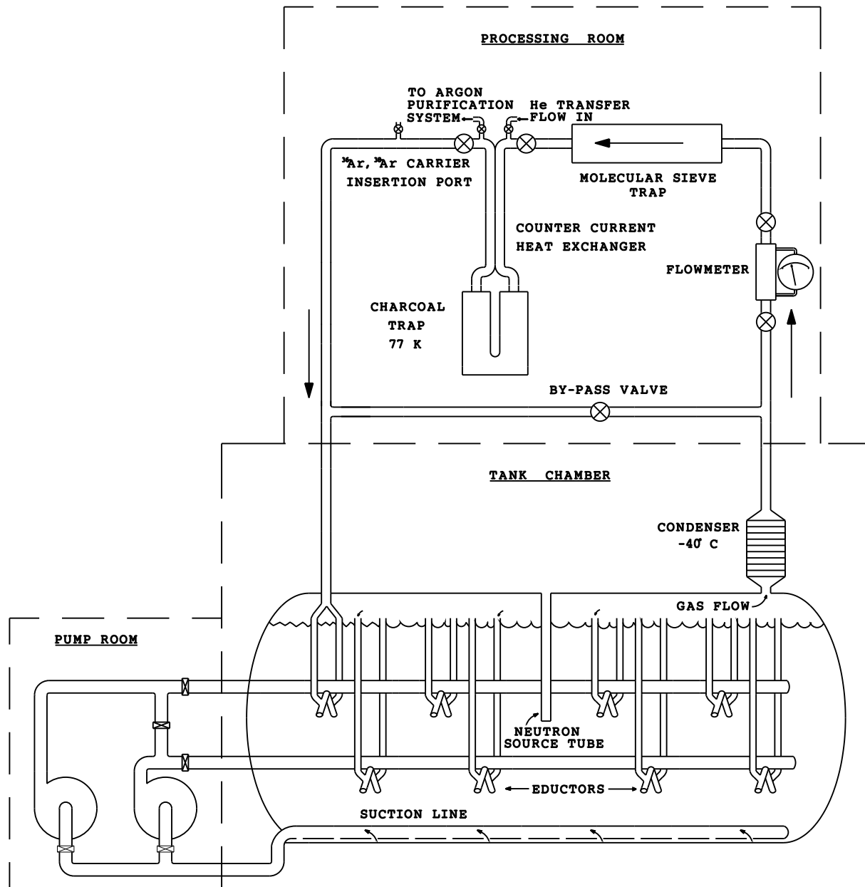
FIG. 2.—Schematic of Homestake solar neutrino experiment. Functional arrangement of the detector elements described in § 3. For purposes of clarity, the drawing shows only four pairs of eductors attached to each header pipe within the C_2Cl_4 tank; there are actually 10 pairs on each pipe.
